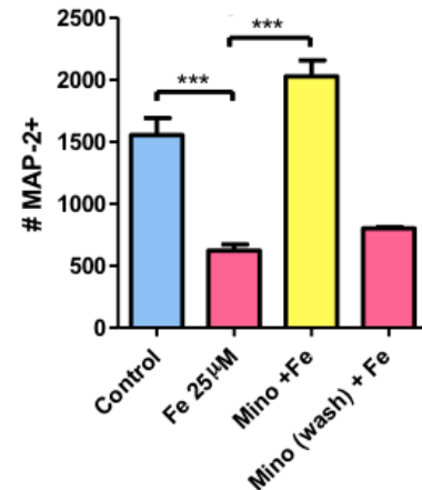
Figure 1. Mean number of MAP-2 positive neurons present in each treatment group (+SEM; n=4). Minocycline concentration is 10µg/mL, and Fe 2+ is a 25µM FeSO 4 challenge. Both minocycline pre-treatment and Fe 2+ challenge times were 24 hours. In the “wash” group, contents of the wells were removed before addition of the next treatment. Data were analyzed using a one-way ANOVA followed by the Bonferroni post-hoc test. ***p>0.001.
